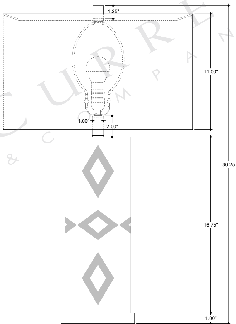
FRONT VIEW
